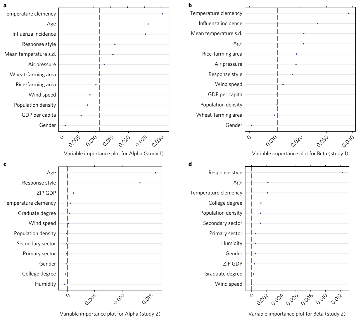
Fig. 3 | Variable importance plots of the predictor variables in machine-learning analyses. a , Alpha (study 1). b , Beta (study 1). c , Alpha (study 2). d , Beta (study 2). The variables to the right of the red dashed line are statistically significant in predicting personality.
